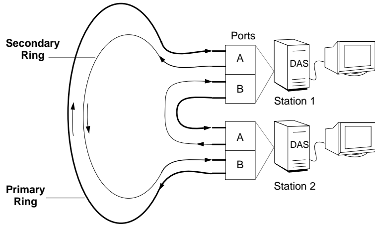
Figure 1-5 Connection of DAS Ports to Primary and Secondary Rings
