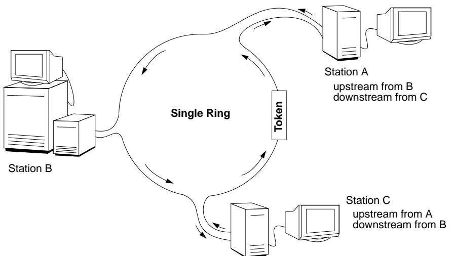
Figure 1-3 Simple Token Ring
