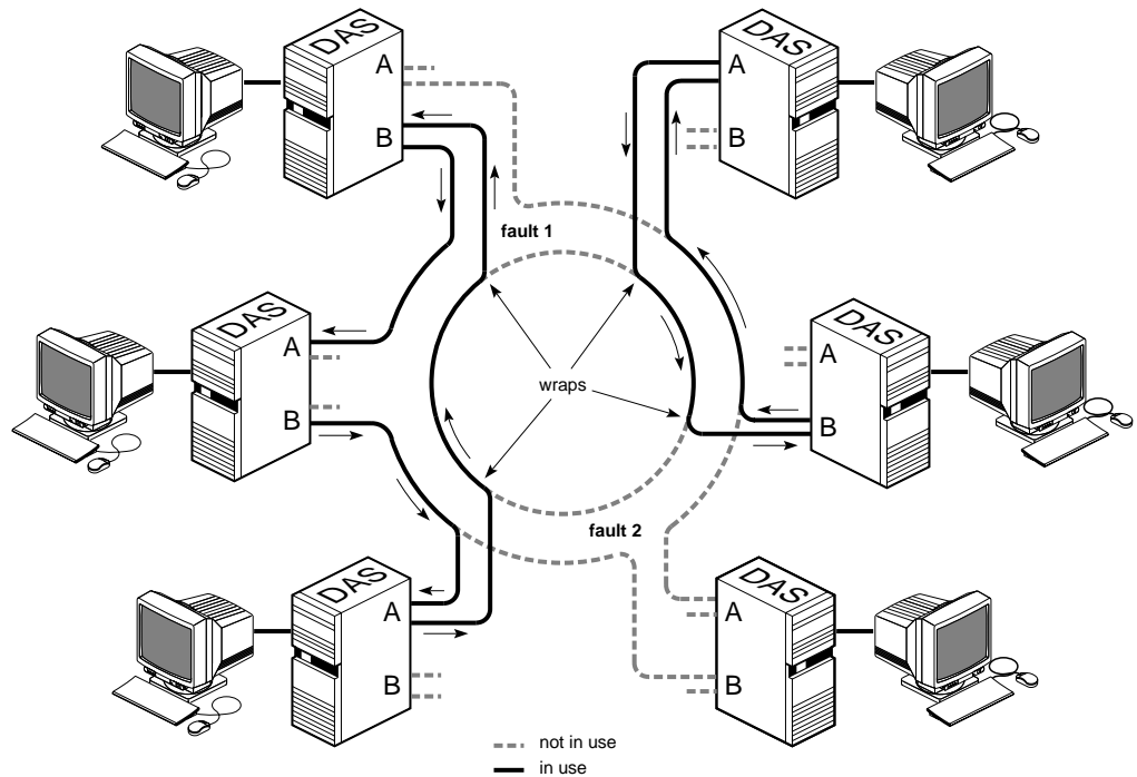
Figure 3-6 A Fragmented Ring
