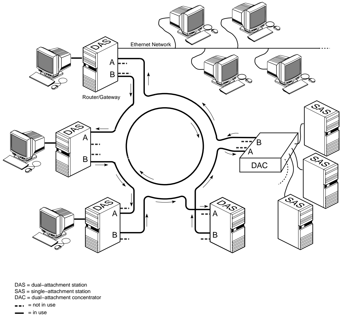
Figure 1-10 FDDI with an Ethernet Network
