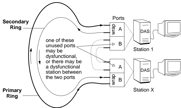
Figure 1-8 Connection of DAS Ports at Points Where Ring Is Wrapped
