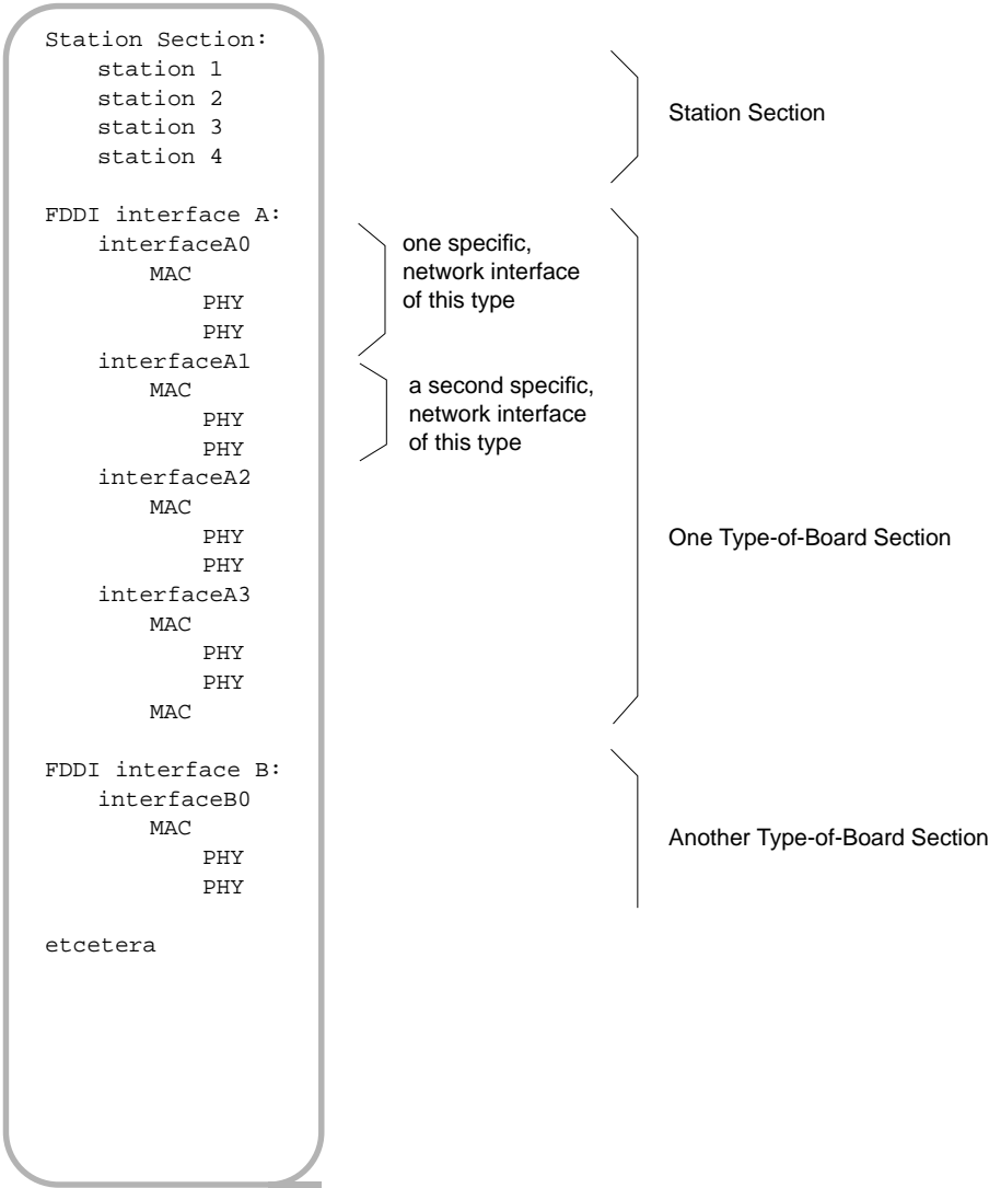
Figure B-1 Outline of smt.d.conf File
