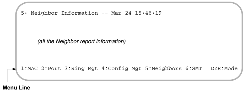
Figure 3-8 smtstat -s Display: General Report Format
