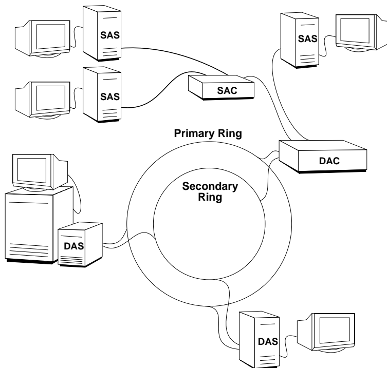
Figure 1-6 An FDDI Ring with Concentrators
