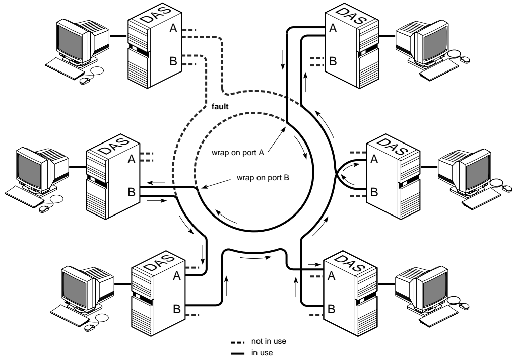
Figure 3-5 Fault Isolation and Ring Wrap
