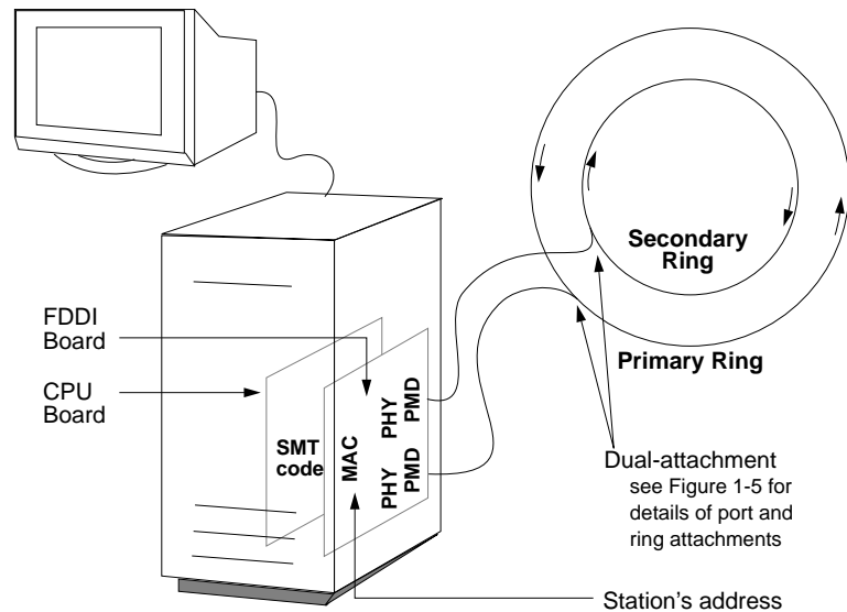
Figure 1-2 FDDI Components of FDDIXPress and an FDDI Board
