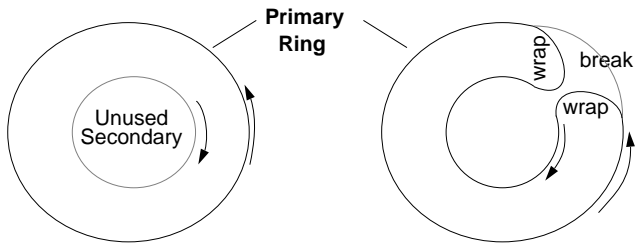
Figure 1-7 Wrapping the Ring
