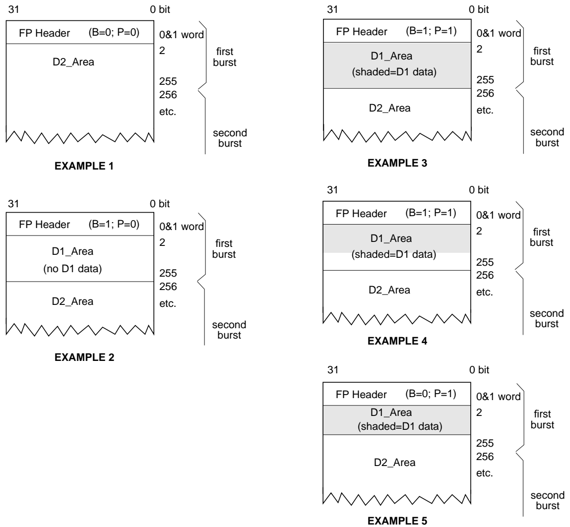
Figure 1-14 Some Common HIPPI-FP Packets
