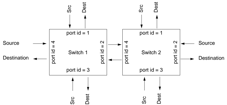
Figure 1-6 Switches and Port Identifiers
