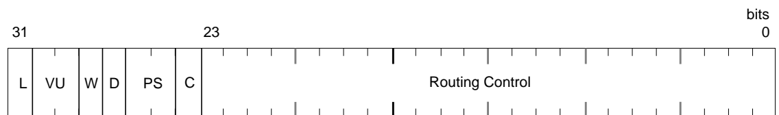
Figure 1-10 I-field Format
