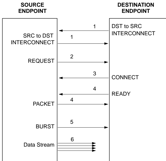
Figure 1-15 HIPPI Signals Used on Each Point-to-Point Link
