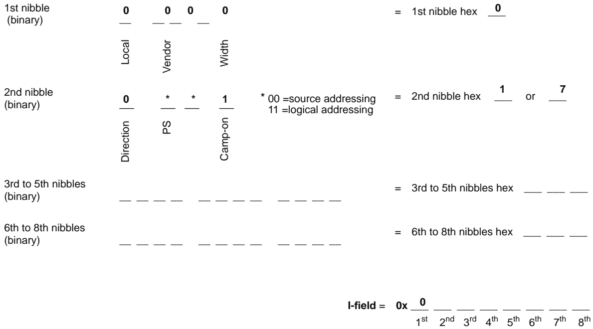
Figure 2-1 Template for Creating I-fields With Recommended Values
