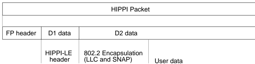
Figure 1-21 HIPPI Packet Created by IRIS HIPPI-LE
