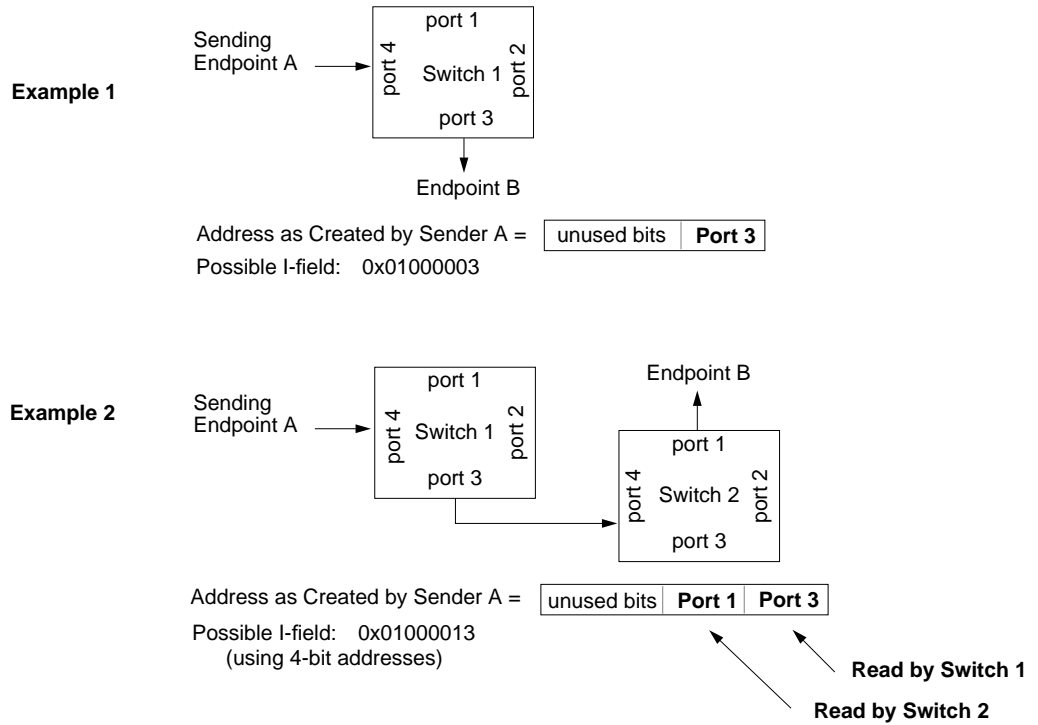
Figure 1-7 Port Identifiers for Source Addressing
