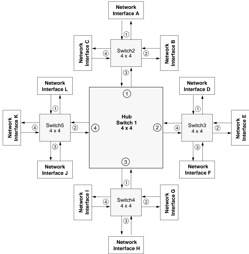
Figure 1-19 HIPPI LAN Configurations With Multiple Switches
