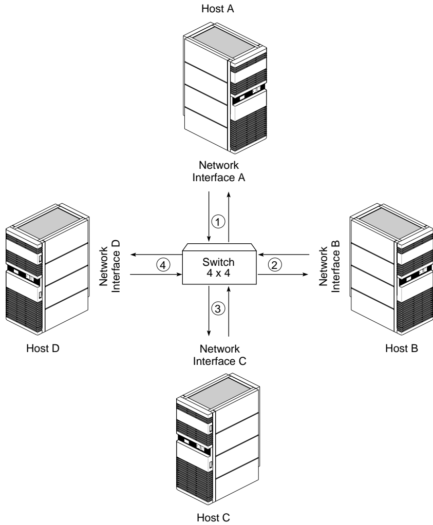
Figure 1-18 HIPPI LAN Configuration With One Switch
