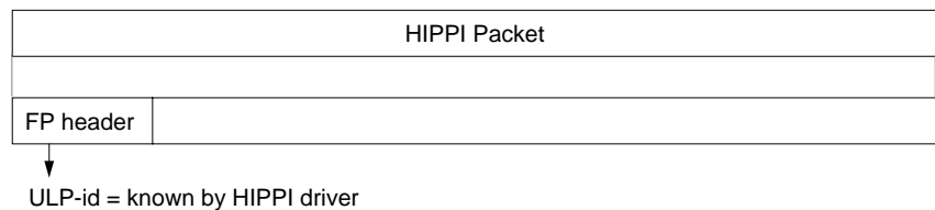
Figure 1-22 HIPPI Packets that IRIS HIPPI Driver Passes to HIPPI-LE
