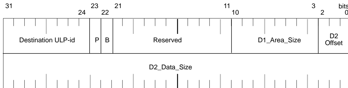
Figure 1-12 FP Header Format
