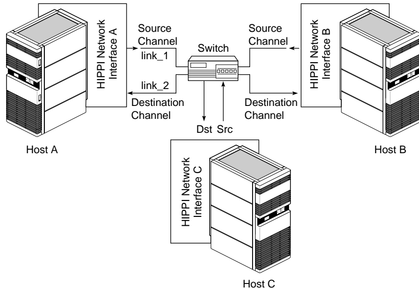
Figure 1-1 HIPPI Links and Connections
