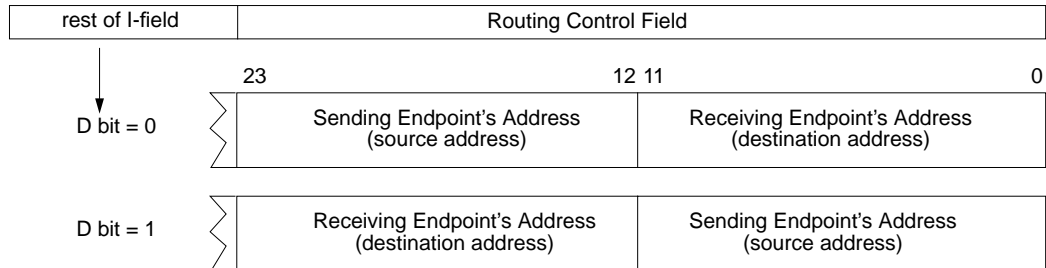
Figure 1-3 Routing Control Field With Logical Addressing
