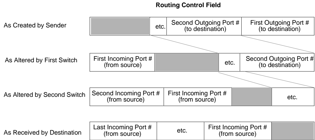
Figure 1-9 How Switches Alter Source Addresses
