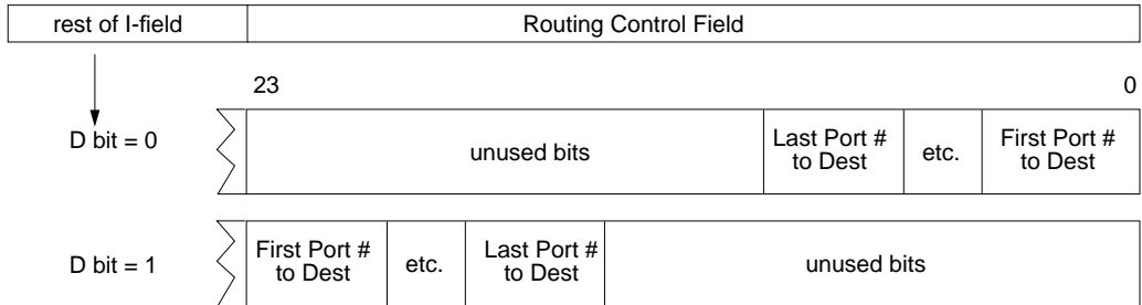
Figure 1-5 Routing Control Field (As Created by Sender) With Source Addressing
