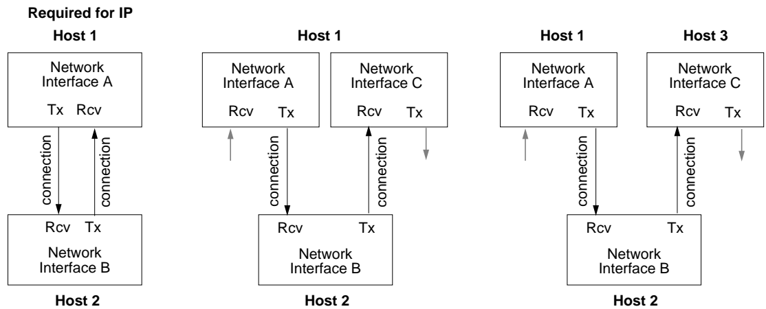
Figure 1-17 Three Variations of the Basic Configuration
