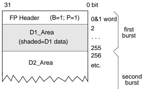
Figure 1-13 Sample HIPPI-FP Packet
