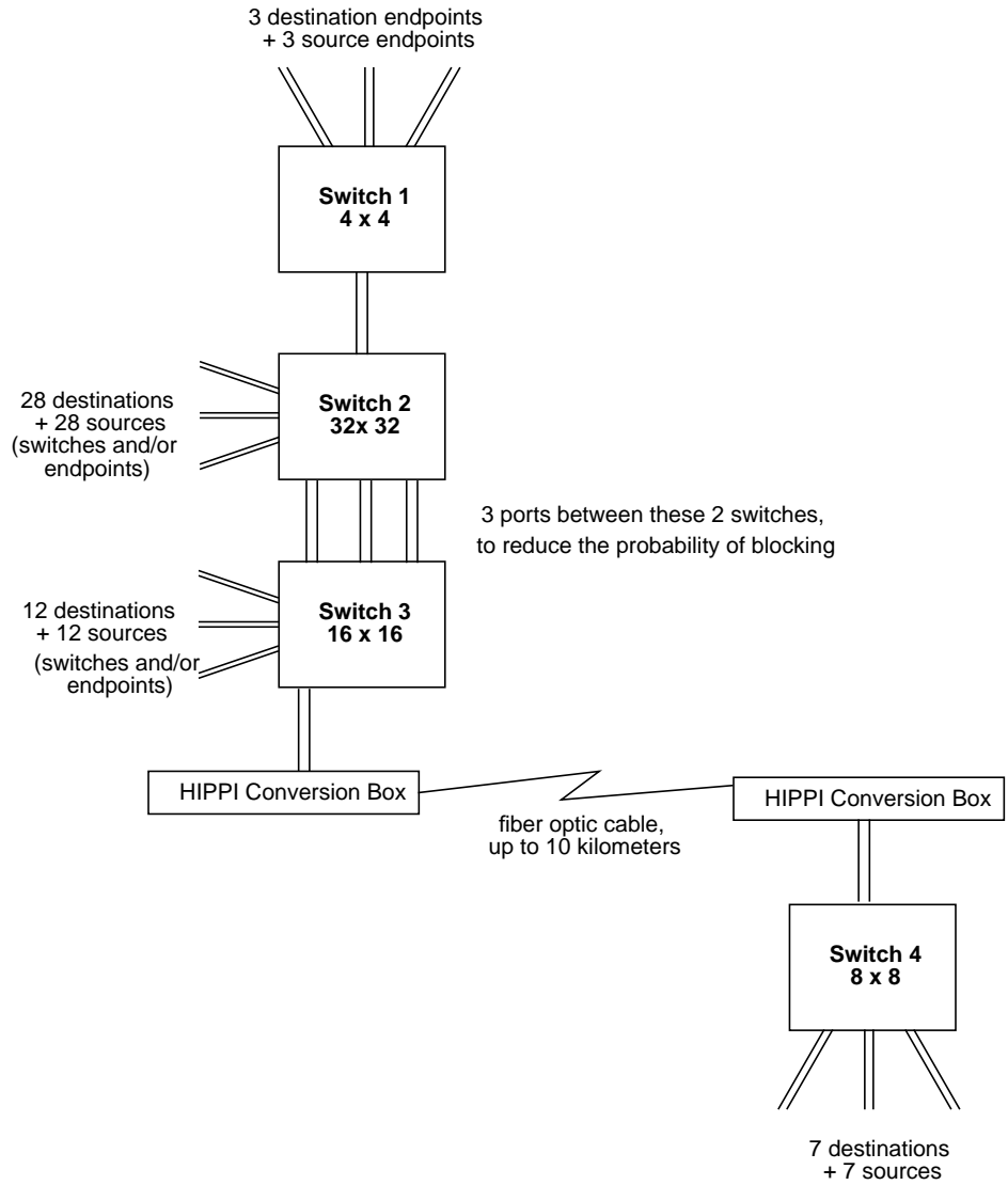
Figure 1-20 Complex HIPPI LAN Configuration
