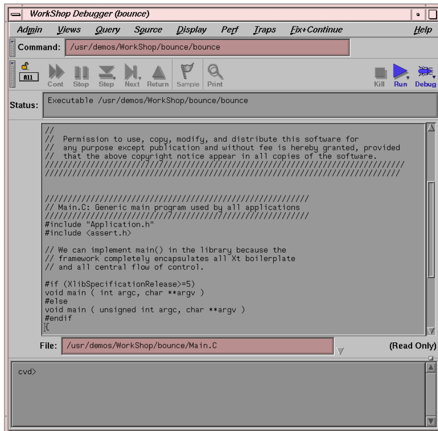
Figure 2-1 The Main View Window
