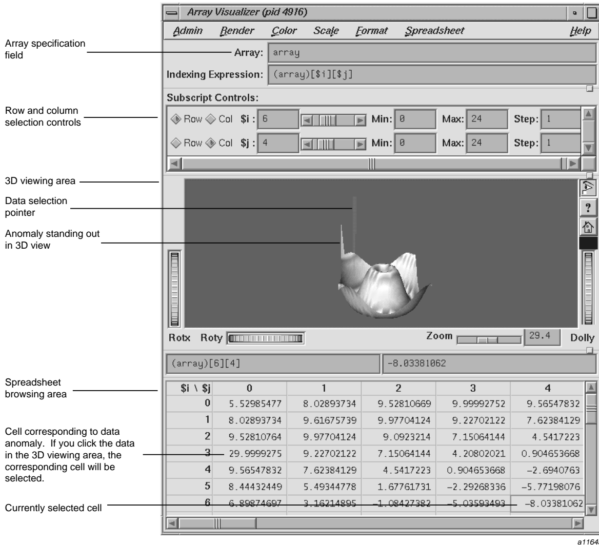
Figure 2-2 Array Visualizer Window
