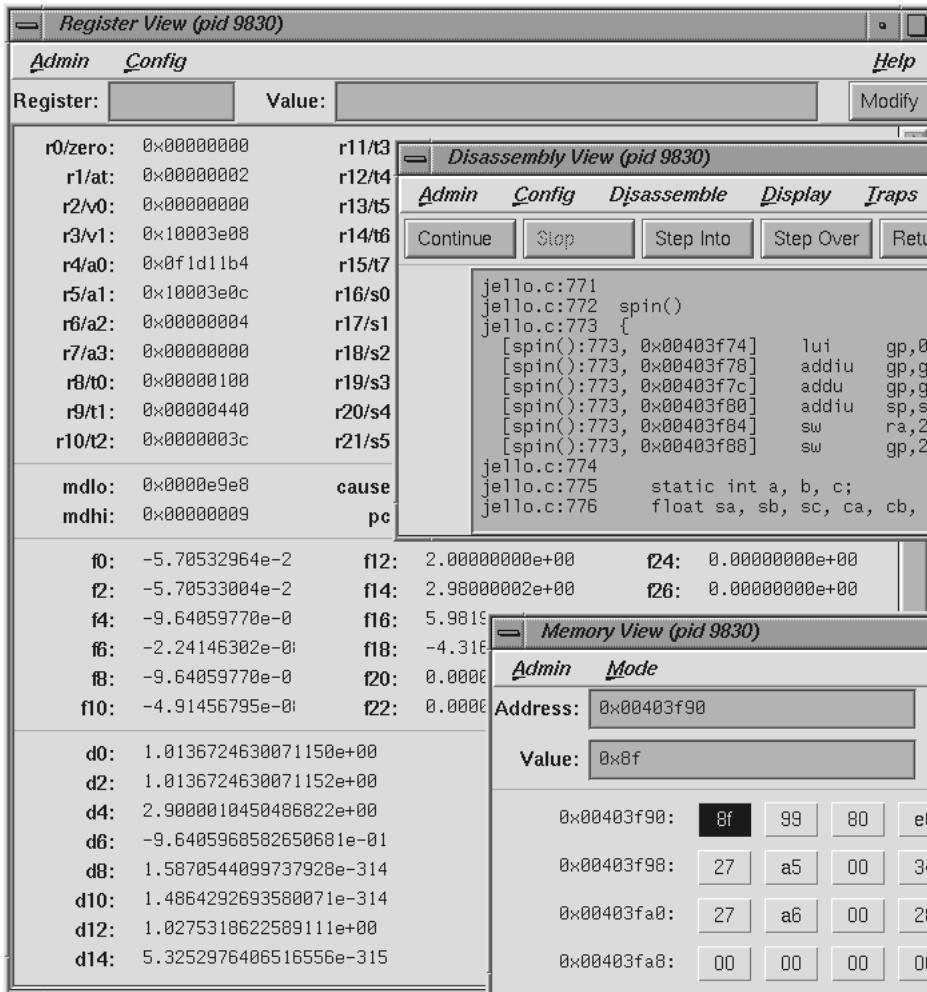
Memory View, for viewing or changing the contents of memory addresses
