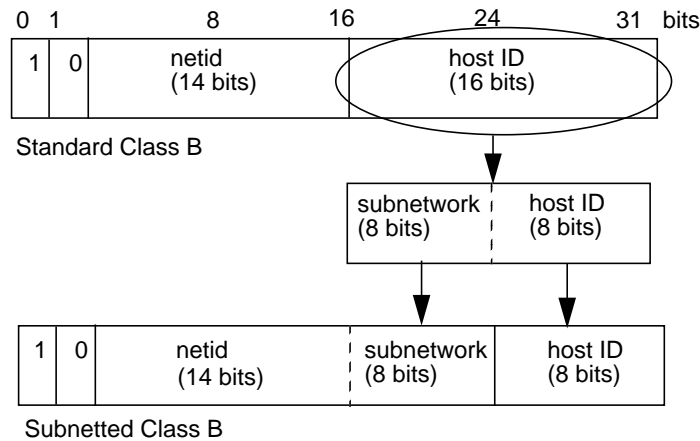
Figure 2-3 Subnetted Class B Address
