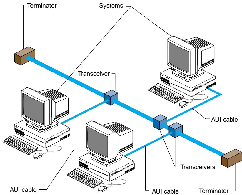
Figure 1-1 Ethernet Network Attachment
