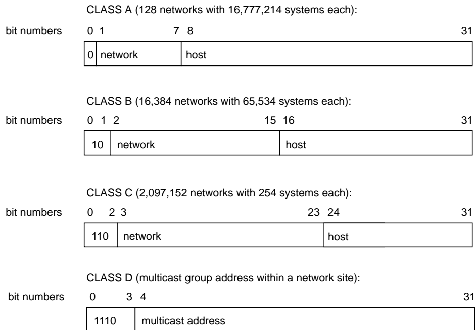
Figure 2-2 The Format of Internet Protocol (IP) Addresses
