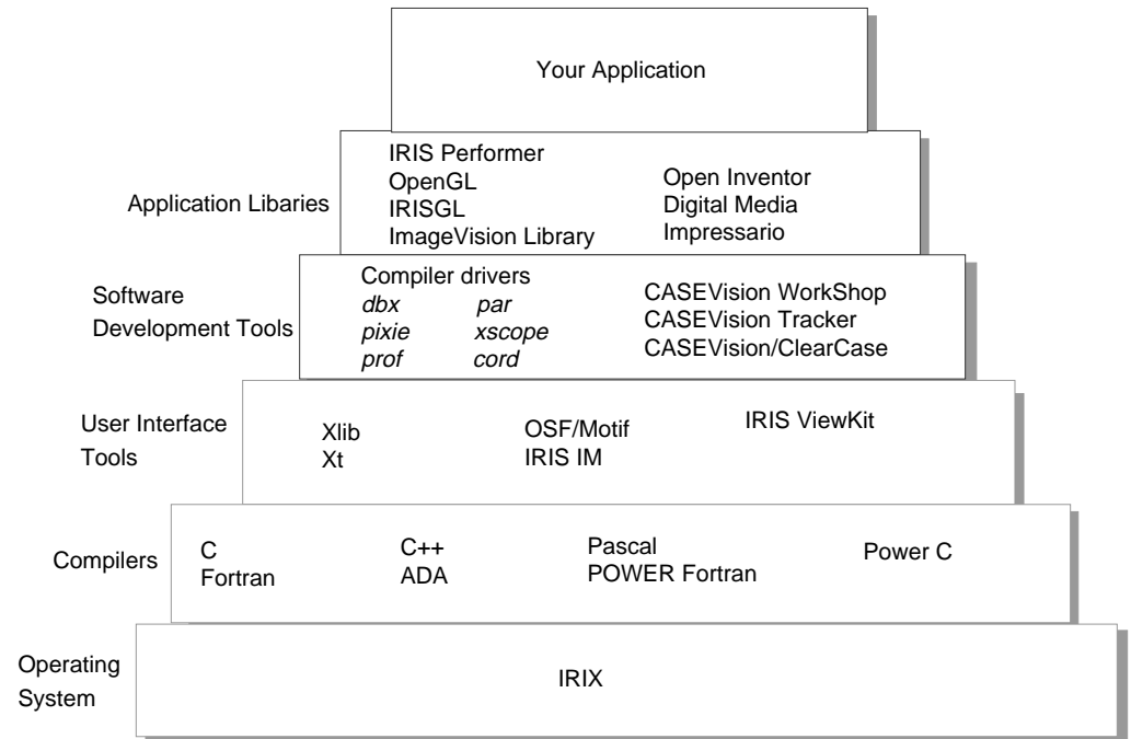
Figure 1-2 Component Hierarchy of an IRIX Application Program
