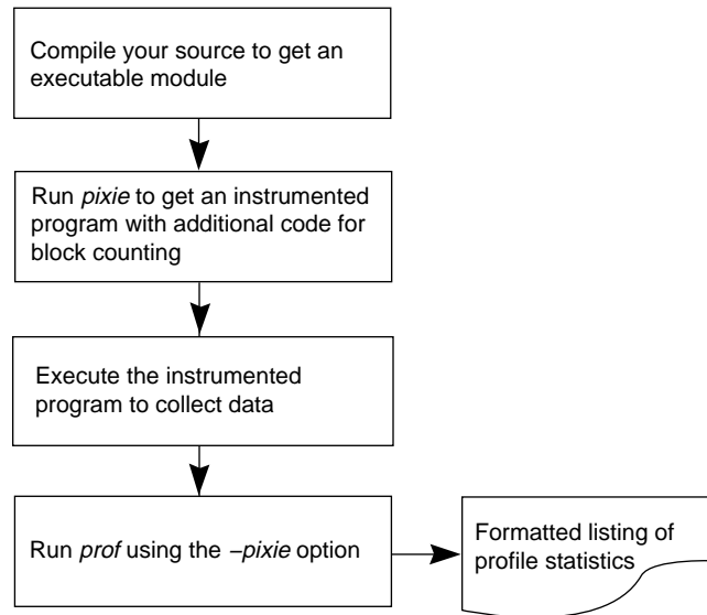
Figure 5-2 Using pixie to Collect Basic Block Counts
