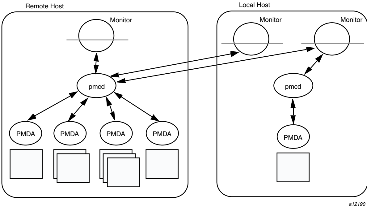
Figure 2. Process Structure for Distributed Operation
