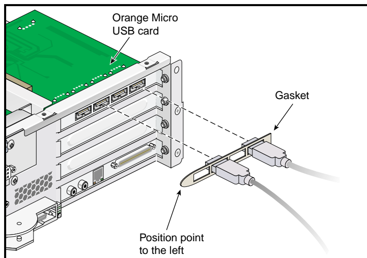
Figure 1 Attaching Gasket to USB Card Bulkhead
