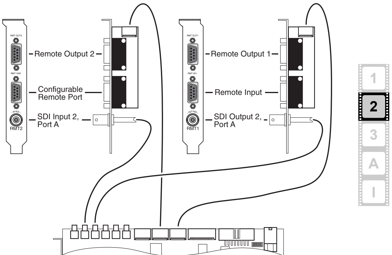
Figure 2-3: RS-422 panel
